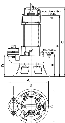
BF-21PN
