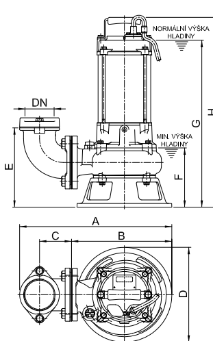
BF-32APN • BF-33APN
